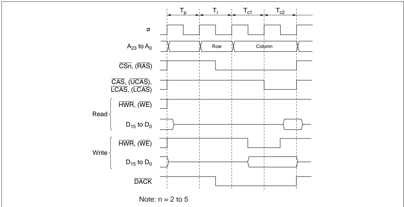
Figure 6-29 \overline{\text{DACK}} Output Timing when \text{DDS} = 0 (Example of DRAM Access)
