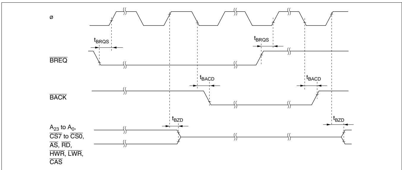
Figure 22-16 External Bus Release Timing
