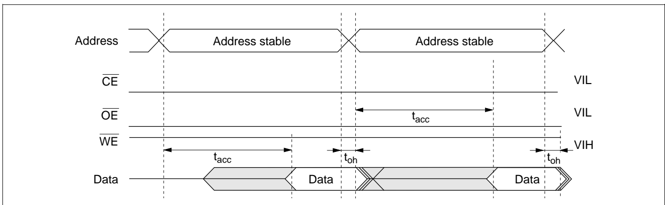
Figure 19-27 Timing Waveforms for \overline{CE}/\overline{OE} Enable State Read
