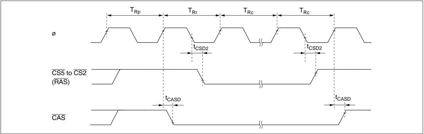
Figure 22-45 Self-Refresh Timing
